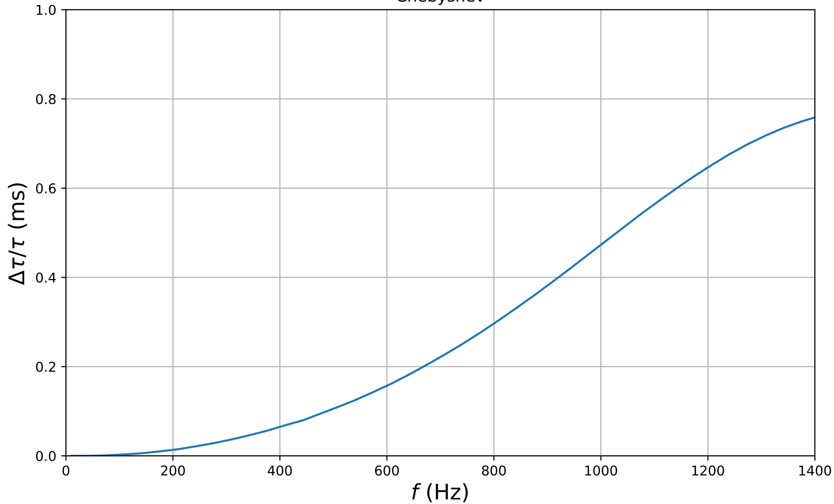
Chebyshev
